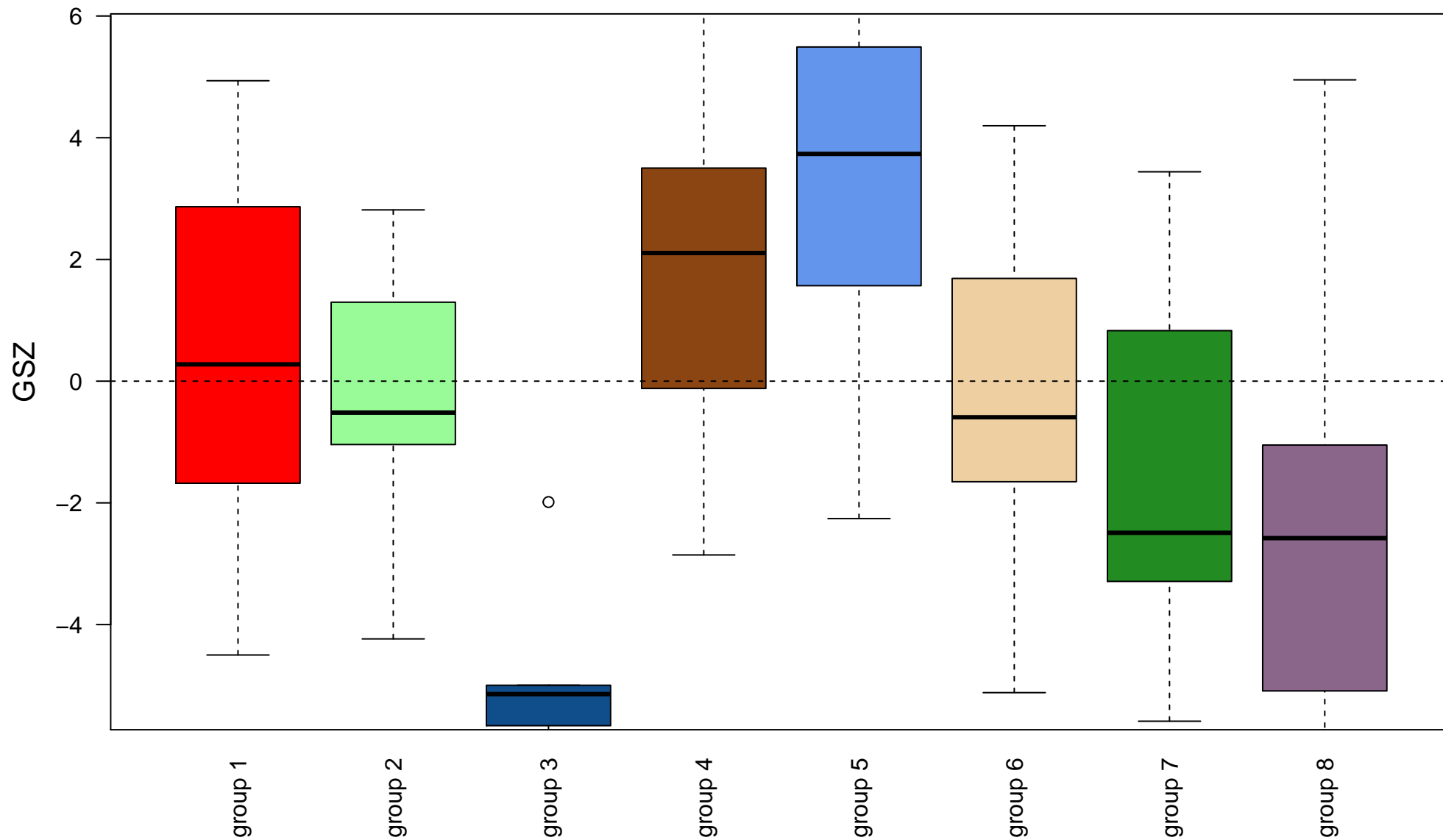
DNA-binding transcription factor activity
